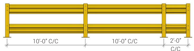
Layout Example (Elevation View)
