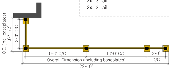
Layout Example (Plan View)
